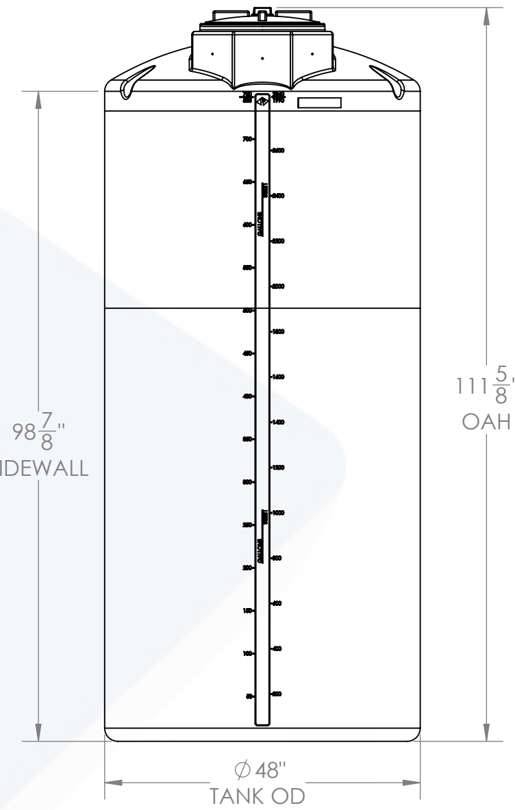
FRONT VIEW
