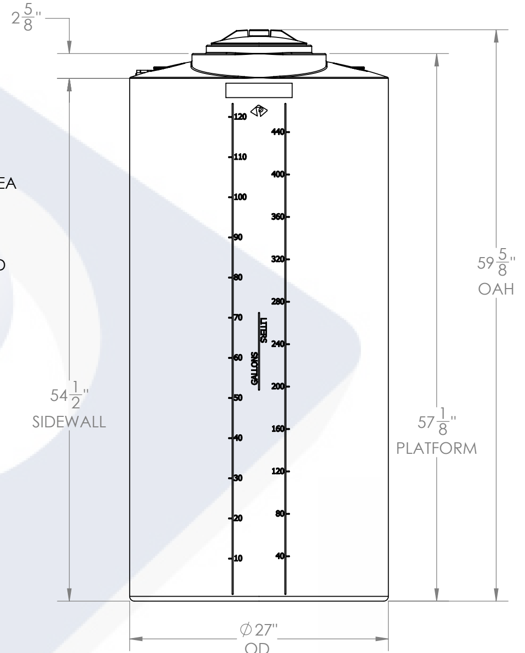
FRONT VIEW
