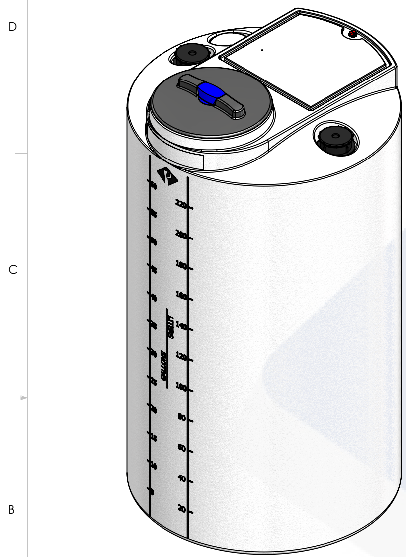
ISOMETRIC VIEW
